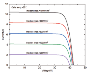
I-V Curves of SPP350NHES at different irradiance
