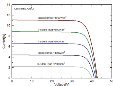
I-V Curves of SPP370QHES at different irradiance
