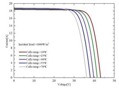
I-V Curves of SSD600YH6H at different cell temperature
