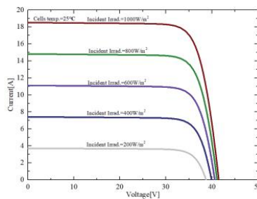
I-V Curves of SSD600YH6H at different irradiance
